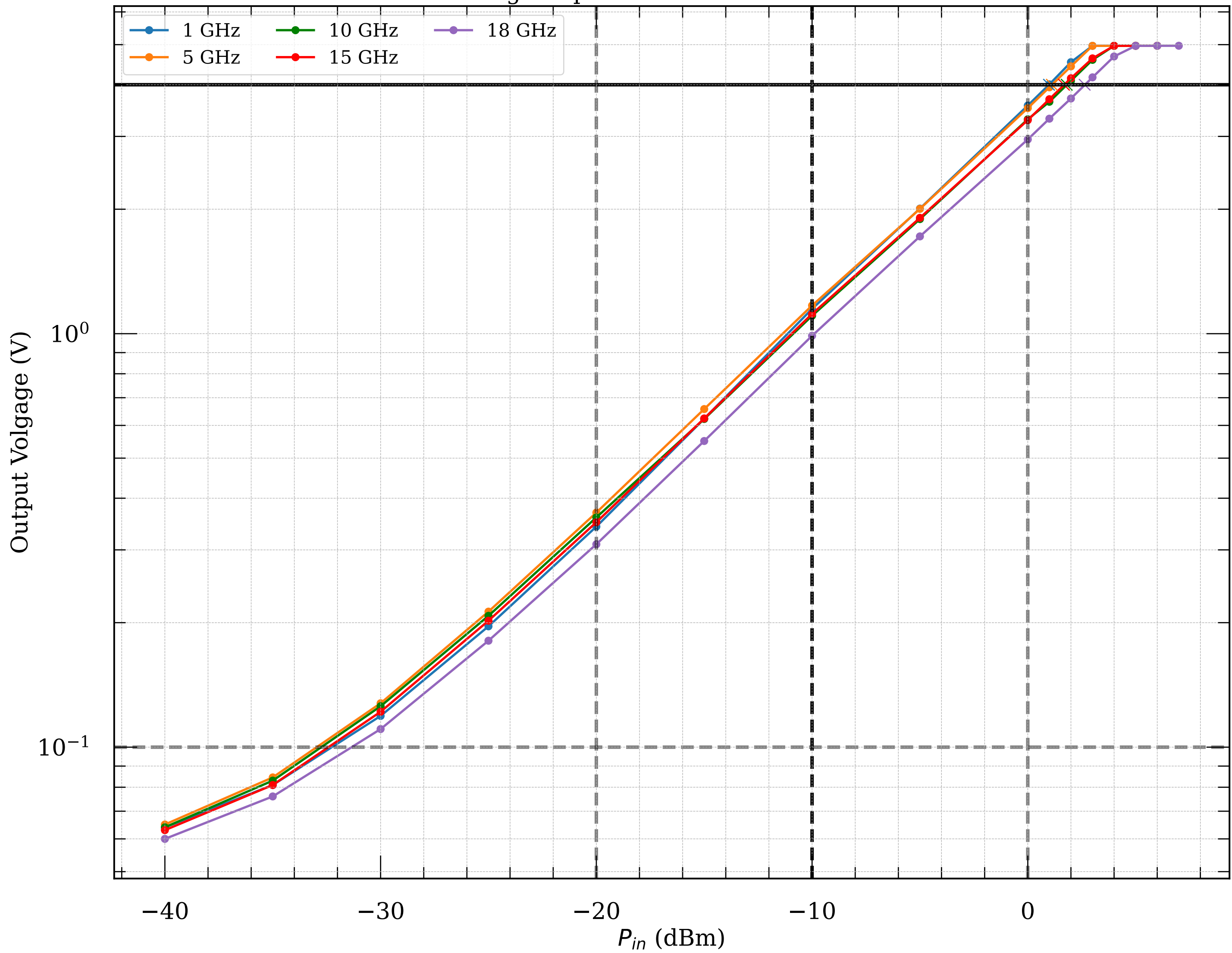
Measured voltage-to-power curve of detector module019v2
